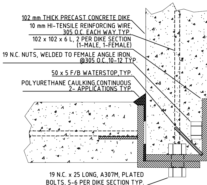
CORNER DIKE JOINT SECTION VIEW
