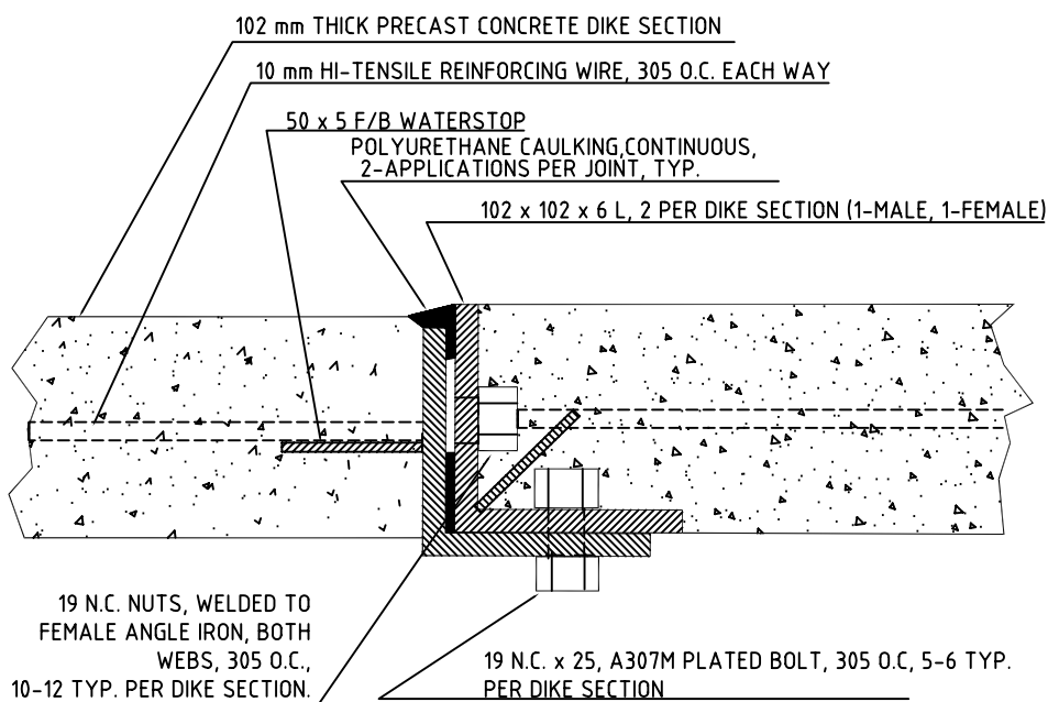
INLINE DIKE JOINT SECTION VIEW
