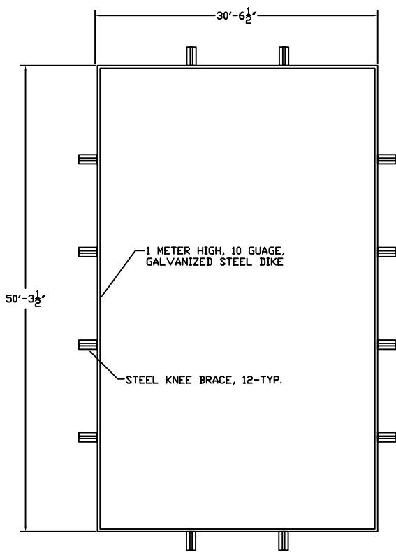
750 BBL STEEL DIKE RECTANGULAR SYSTEM
