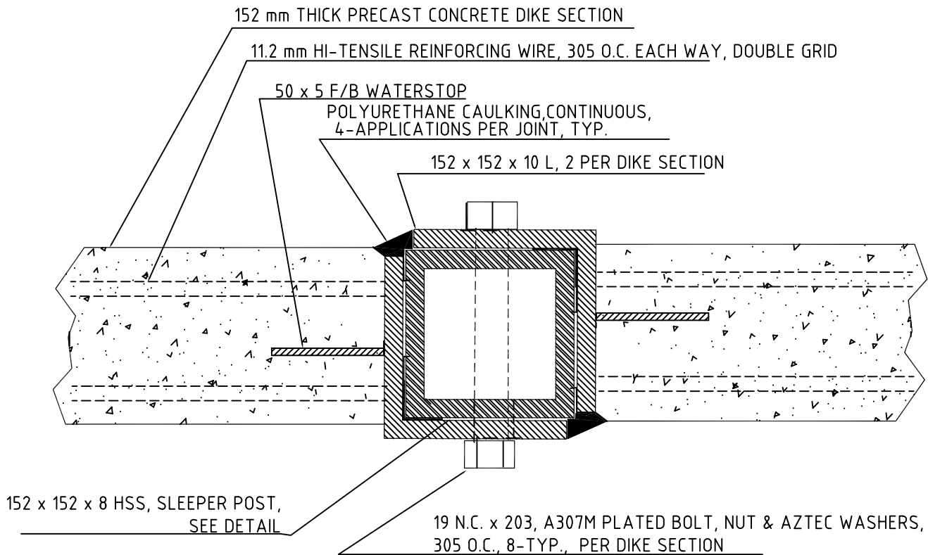
INLINE DIKE JOINT SECTION VIEW
