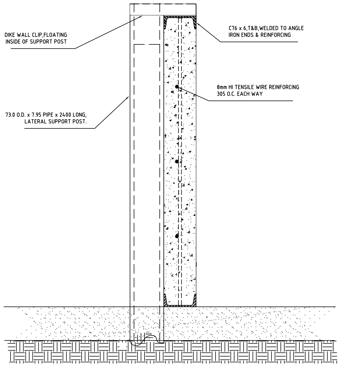
TYPICAL SECTION VIEW
