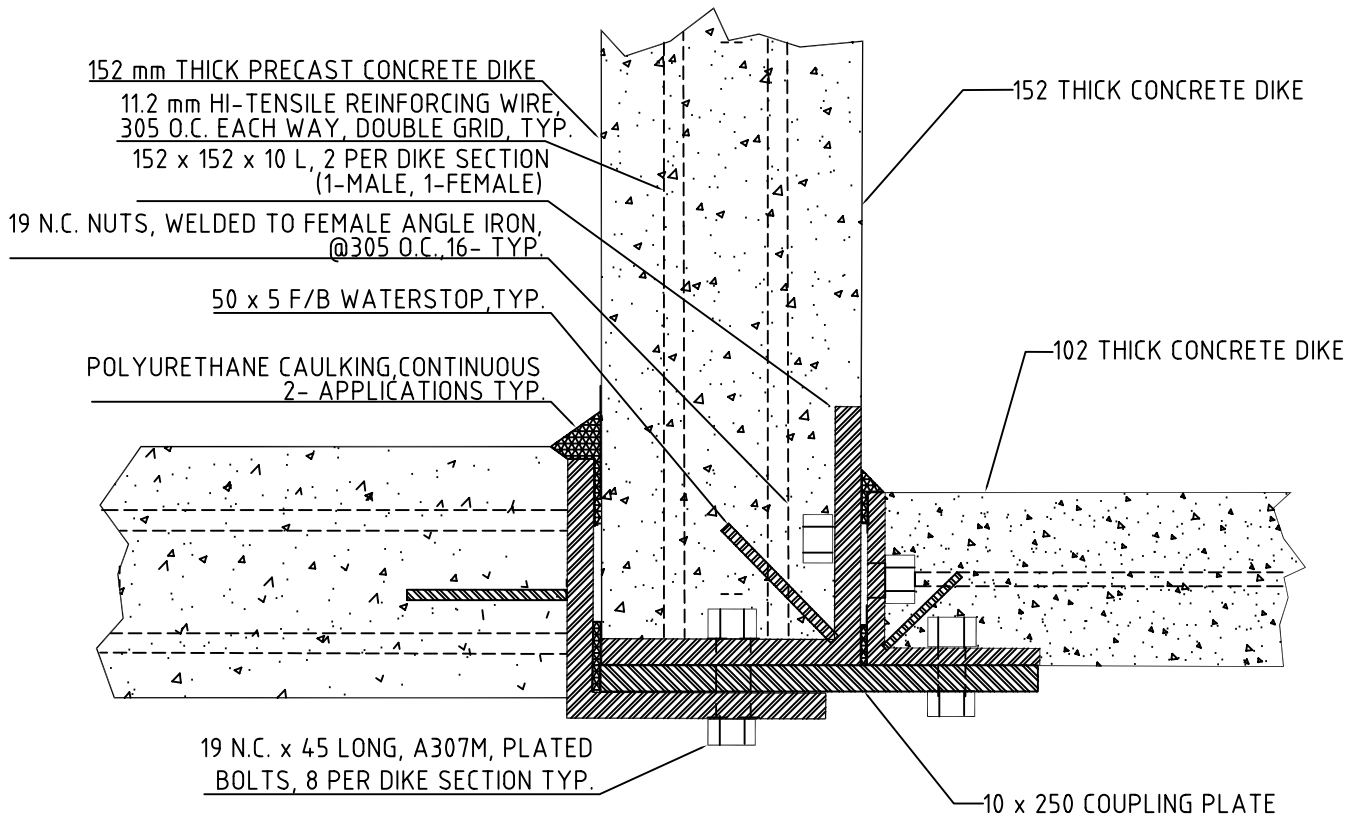
CORNER DIKE JOINT SECTION VIEW
