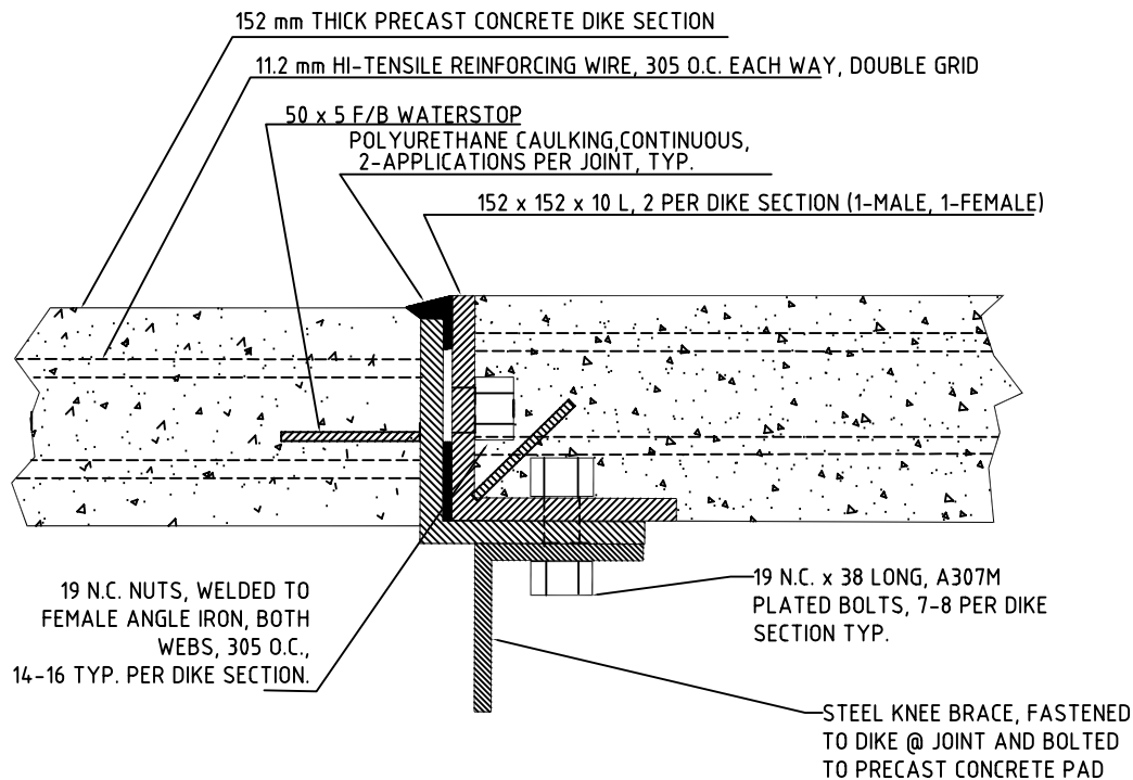
INLINE DIKE JOINT SECTION VIEW
