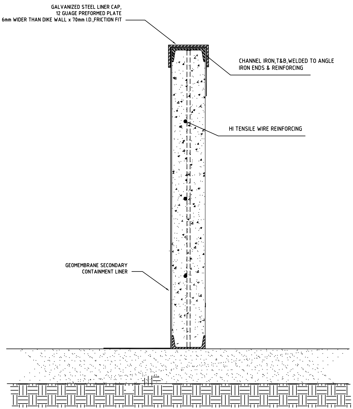
TYPICAL SECTION VIEW
